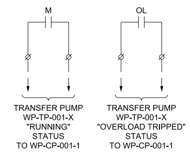
TRANSFER PUMP WP-TP-001-X MOTOR STARTER WIRING DETAIL (X = 2 AND 4)
