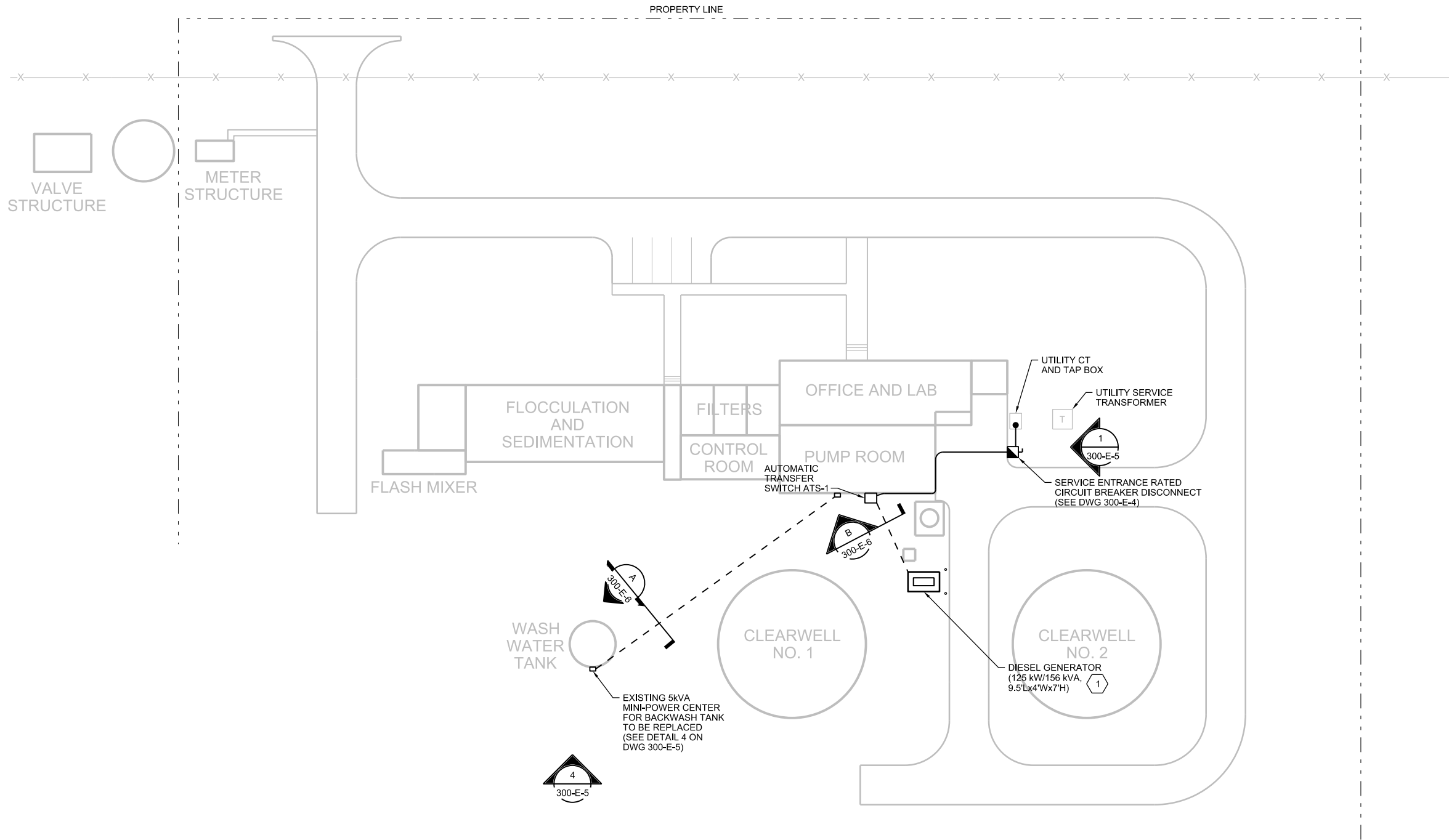
SITE PLAN 1"=30'-0"
